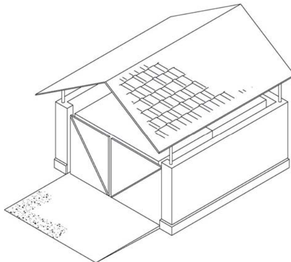
TRASH ENCLOSURE OVERALL VIEW
