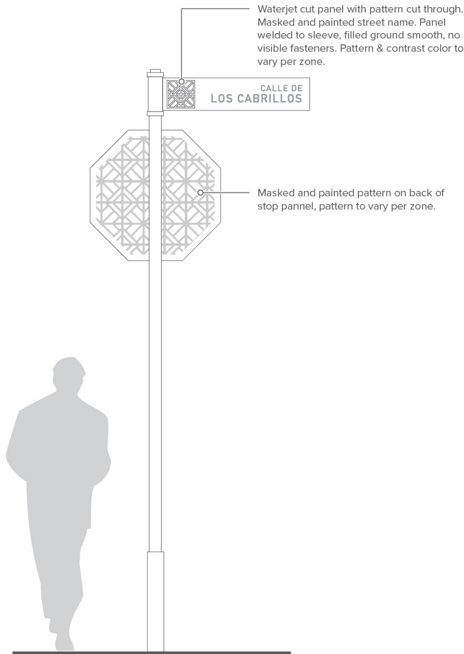
4 Back View Scale : 1/2"=1'
