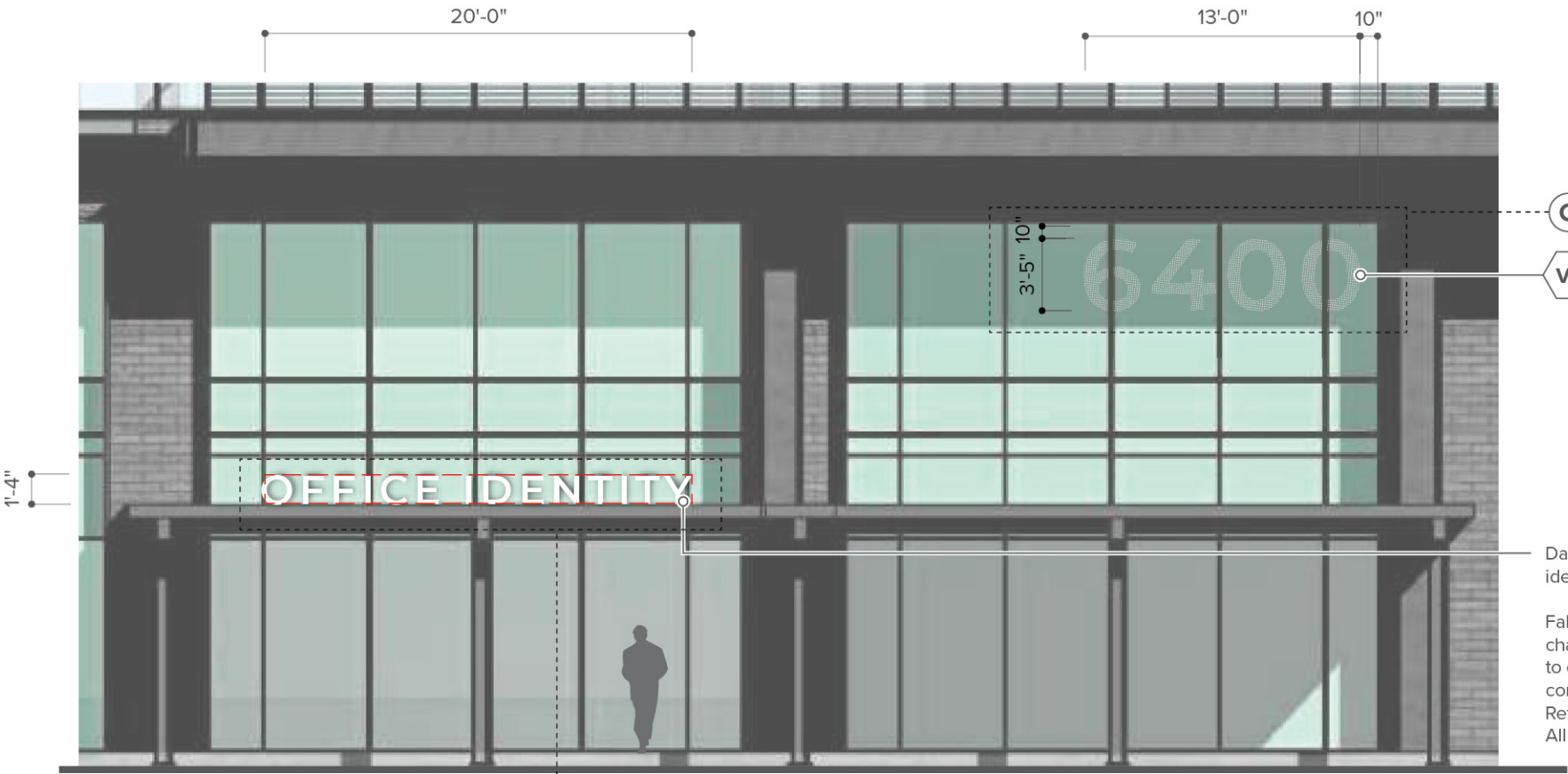
2 Front Elevation Scale : 1/8"=1'
