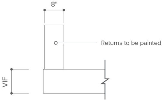
4 Side View Scale : 1/2"=1'
