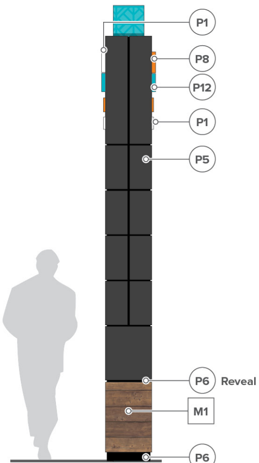
3 Side View Scale : 3/8"=1'
