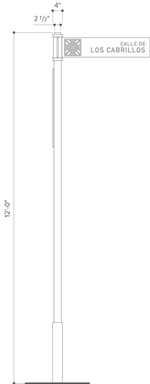
3 Side View Scale : 1/2"=1'
