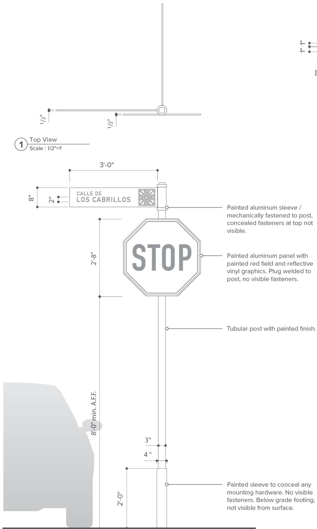
2 Front View Scale : 1/2"=1'
