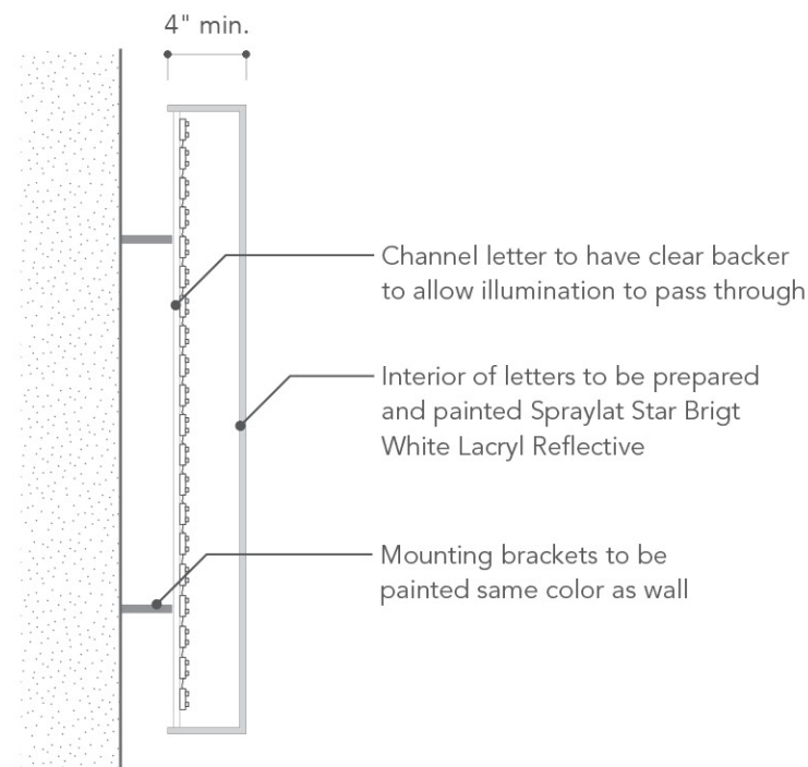
1 Detail of Halo Illuminated letter Scale: NTS
