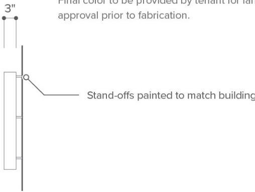
6 Side View Scale: 1/2" = 1'
