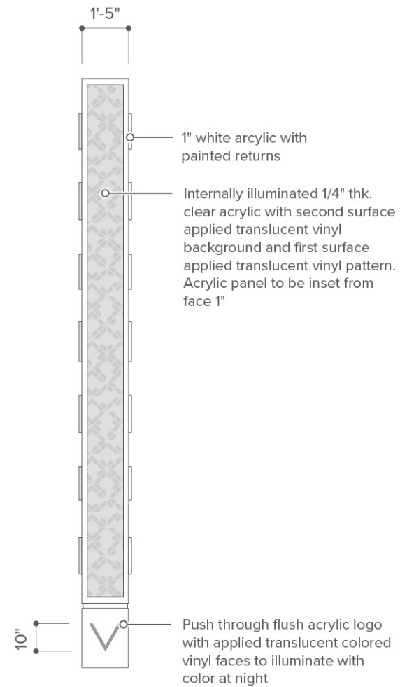
3 Side View Scale : 1/4"=1'
