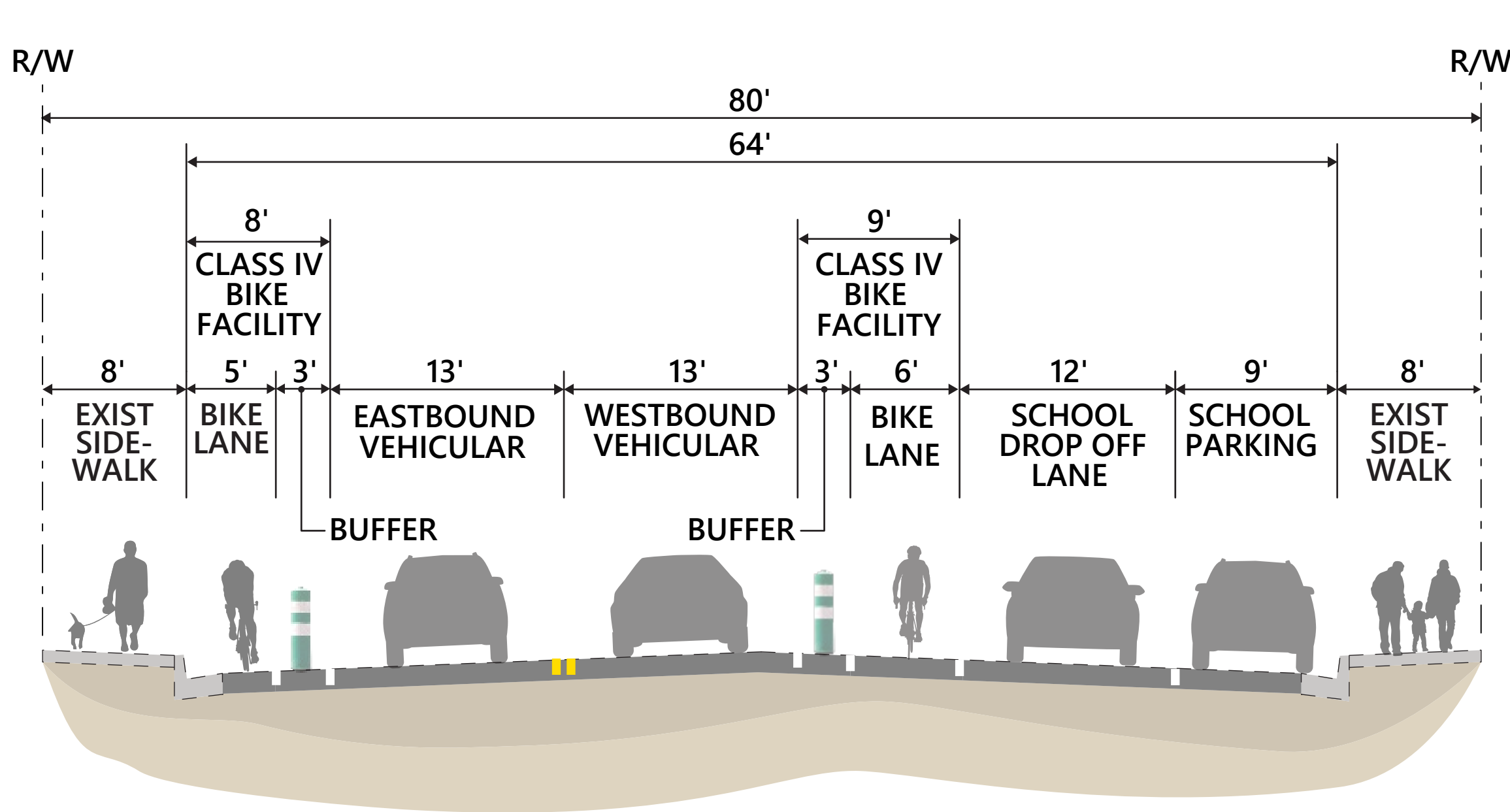
SECTION B-B
