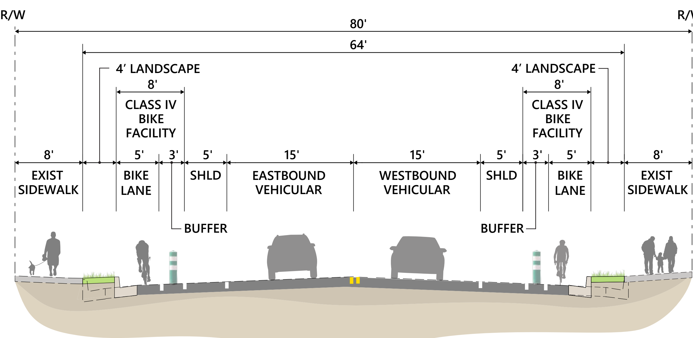
SECTION C-C
